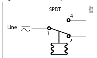
Figure 10: Contact system
